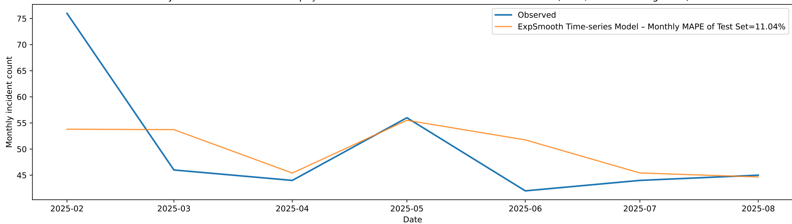
Monthly Traffic Incidents in Mürselpaşa Boulevard: Best Time-series Model vs Observed (TEST, Feb 2025-Aug 2025)
